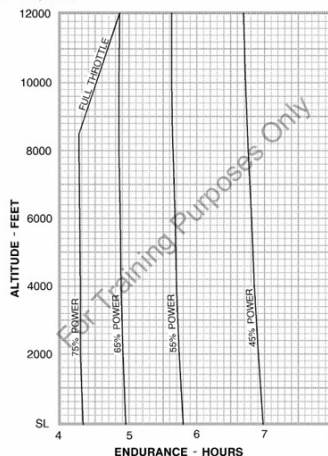
Figure 5-10. Endurance Profile
